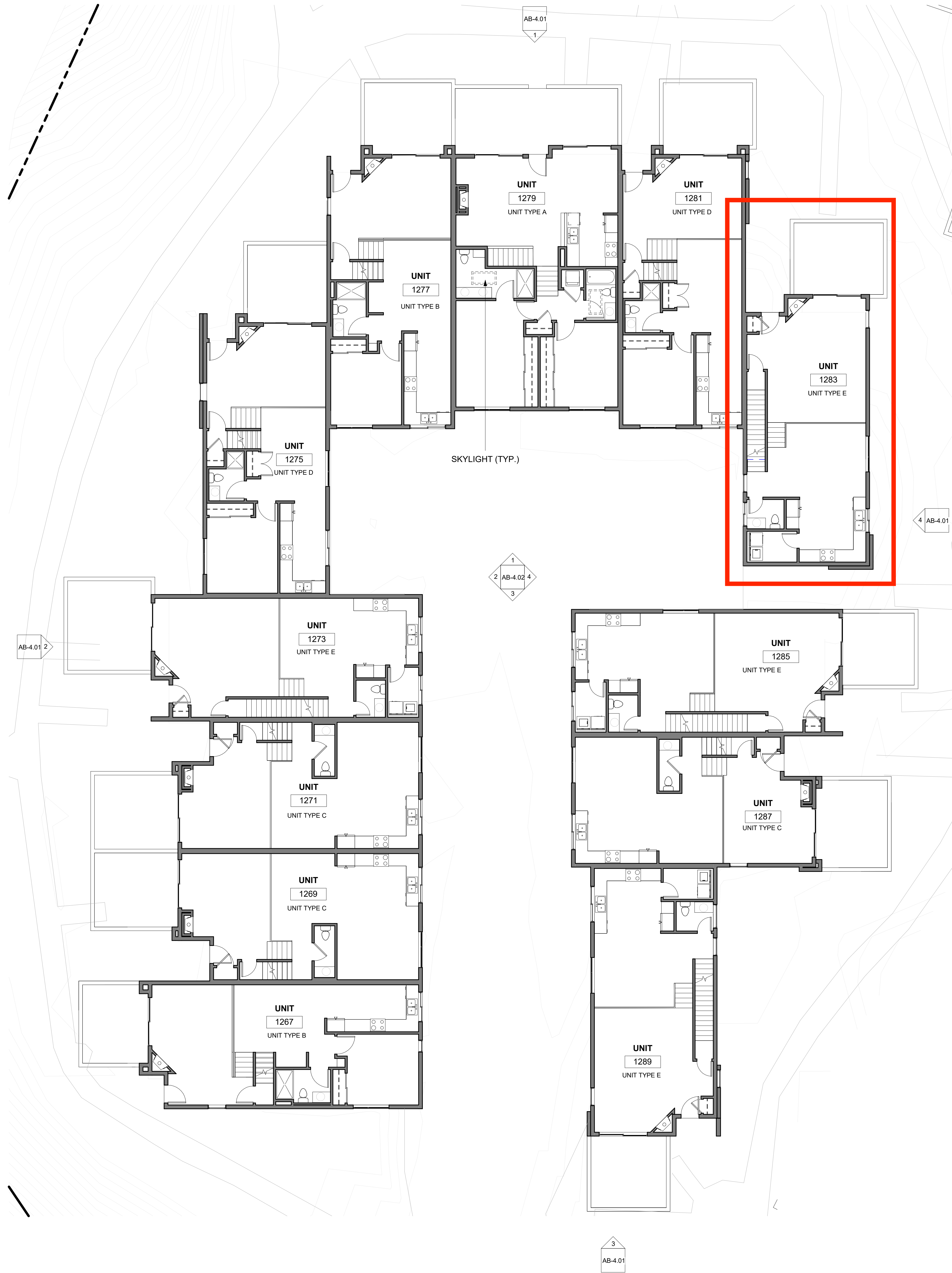
1ST FLOOR/GROUND LEVEL @ BLDG 8
