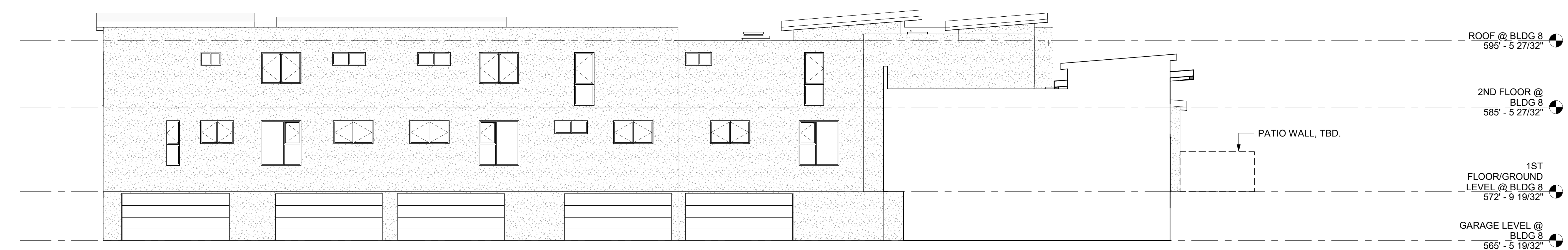
B8 COURTYARD EAST ELEVATION SCALE: 1/8" = 1'-0" 2
