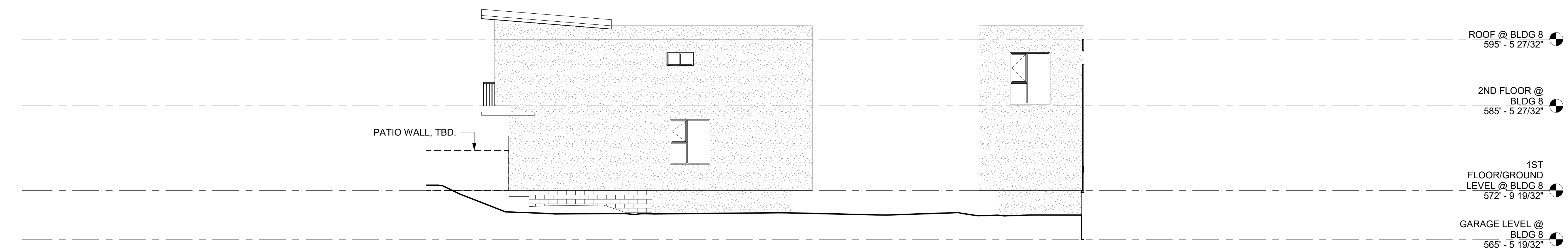
B8 COURTYARD WEST ELEVATION
